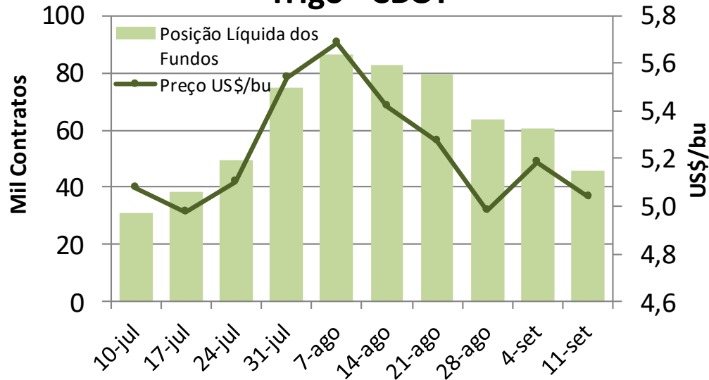
Trigo - CBOT
