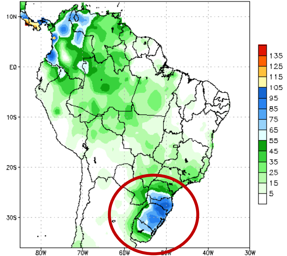
NCEP GFS Ensemble Forecast 8–14 Day Precipitation (mm) from: 23Sep2018 30Sep2018–06Oct2018 Accumulation
